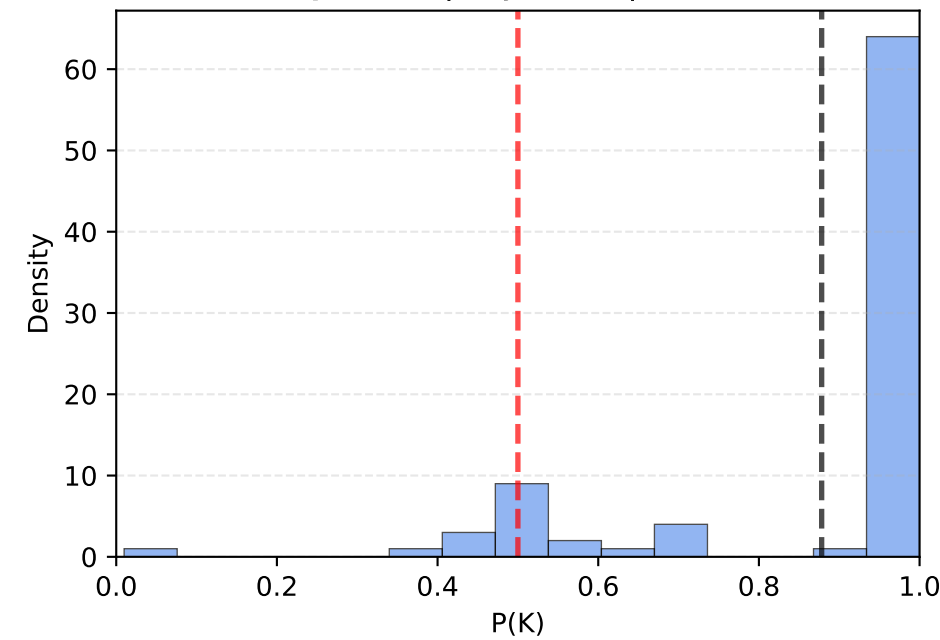
J(K vs R) - Combined \mu : 0.878 | Obj: 0.500 | n=86
